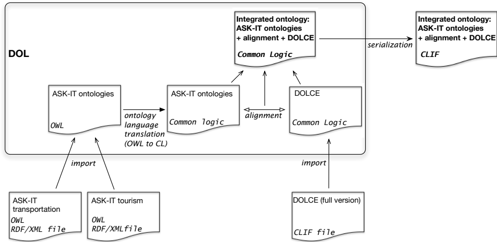
Figure 7.2.: Mapping between two OMSs formulated in different OMS languages
